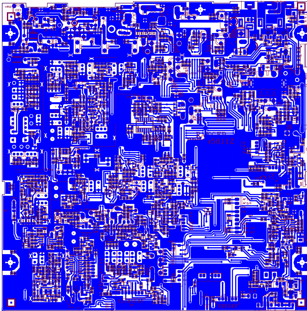
RCI-2950 DX / RCI-2970 DX MAIN PCB
